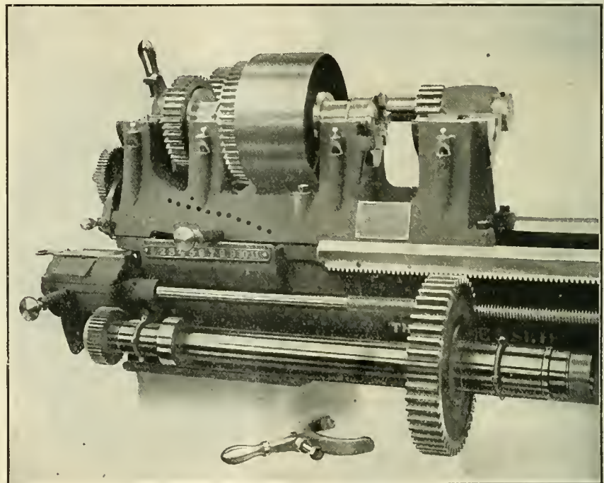
NEW LODGE & SHIPLEY PATENT LATHE HEAD.
